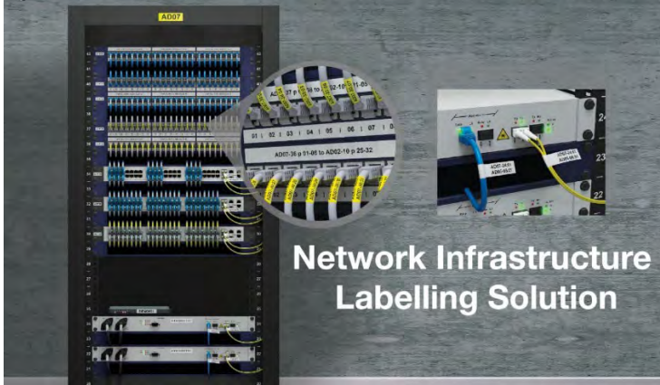
LABELLING (UTP Patch Cord Labelling with PANDUIT Standard)
