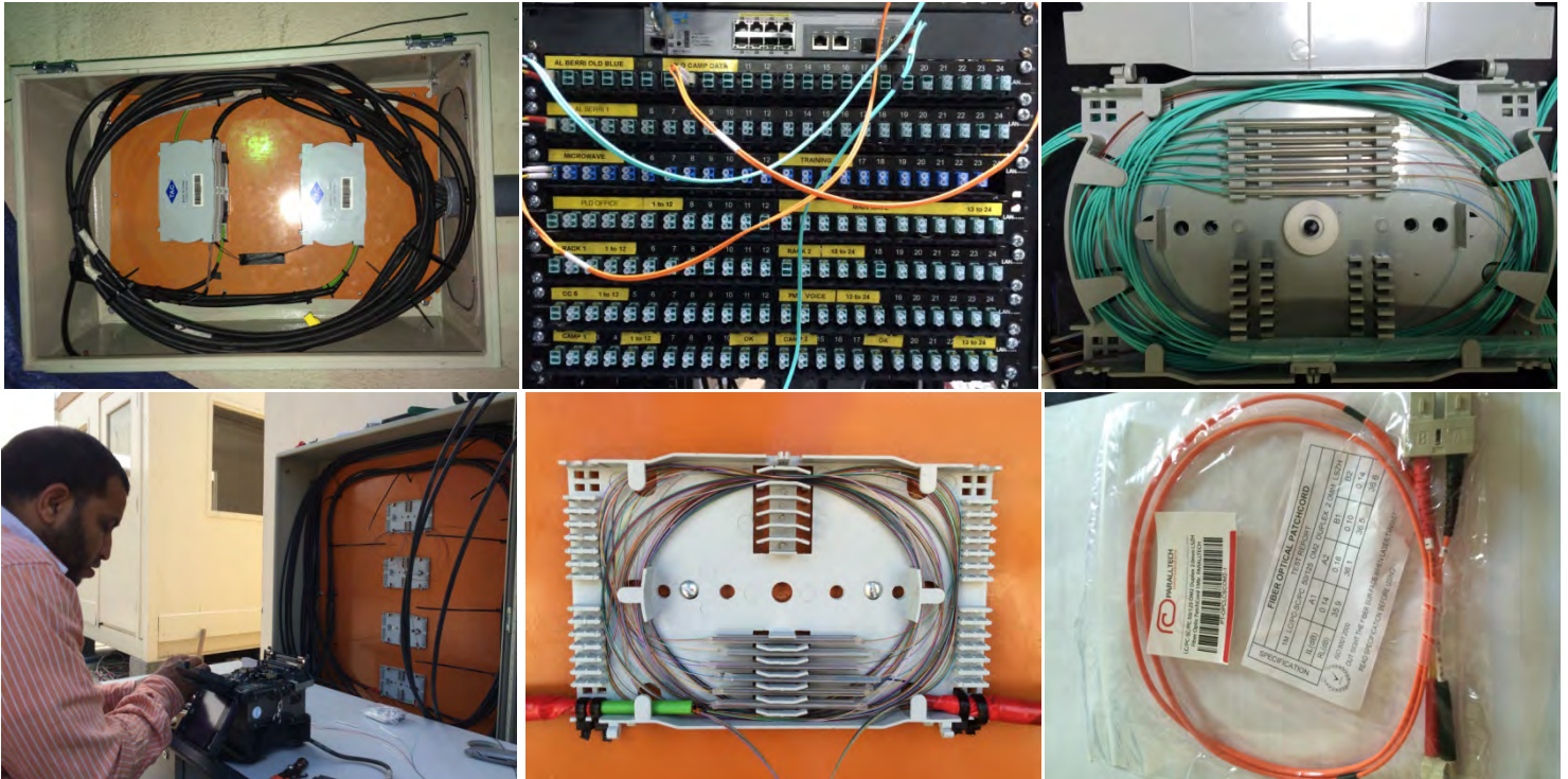
Fiber Optic Splicing (ANABEEB Jubail)
