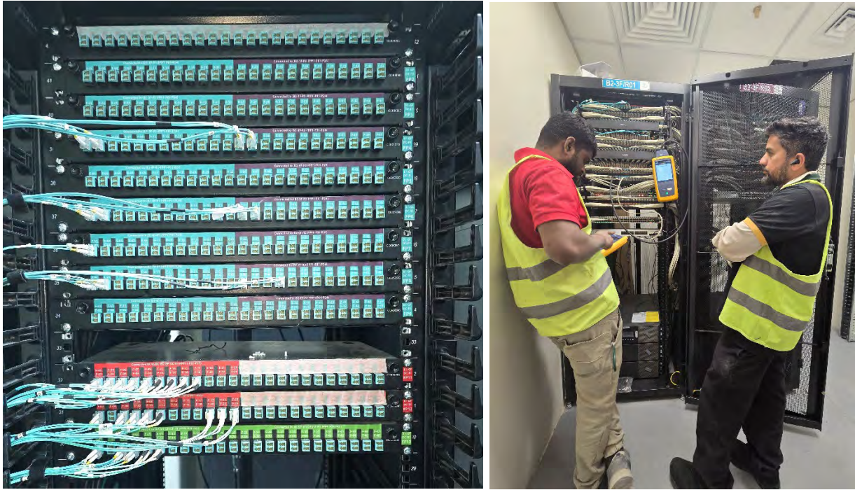
TAHAKOM HEAD OFFICE Riyadh (FIBRE OPTIC PATCH PANELS DATA CENTER & FLUKE TEST AT IDF RACK)
